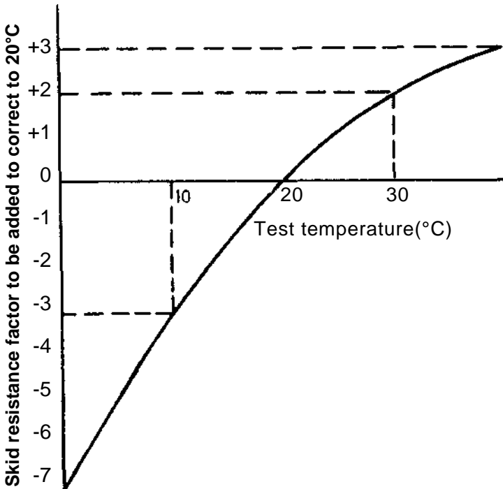
Fig. 1. Suggested temperature corrections for 'skid-resistance' values to allow for changes in resilience of the slider rubber
