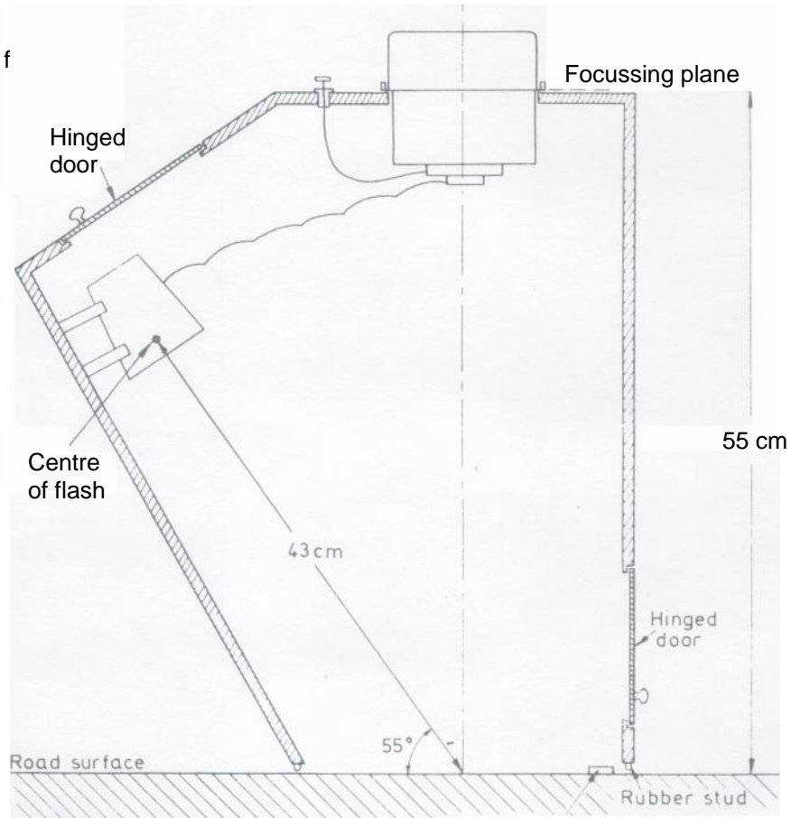
fig. 3. Diagrammatic arrangement of surface texture camera unit
